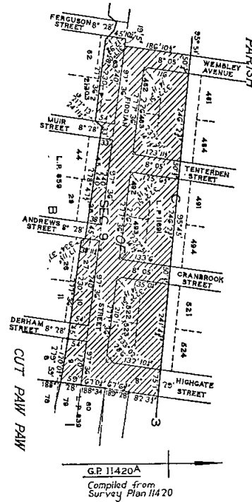
BY-PASS ROAD LOWER YARRA FREEWAY BY-PASS ROAD CITY OF FOOTSCRAY Measurements in feet & inches
