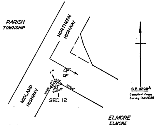
STATE HIGHWAY MIDLAND HIGHWAY SHIRE OF HUNTLY Measurements in links
