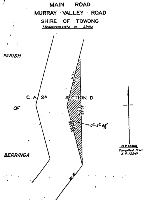
The land shown hatched on Plan numbered G.P.12941 hereunder required for the widening of the Murray Valley road in the Shire of Towong and making of the widening thereon.
