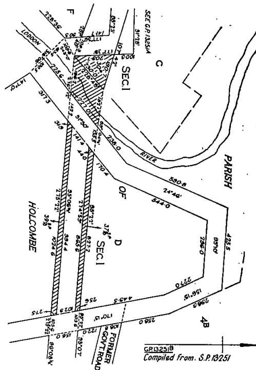
FOREST ROAD DRUMMOND - VAUGHAN ROAD SHIRE OF DAYLESFORD & GLENLYON Measurements in Links
