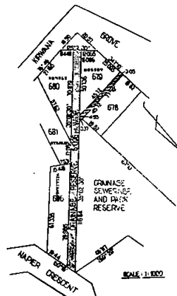
PLAN OF DRAINAGE RESERVE
