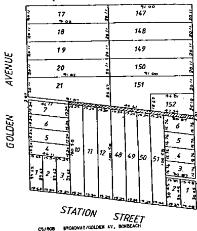
PART L.P.'s 5350, 5351 & 8905. Scale 1:1500
