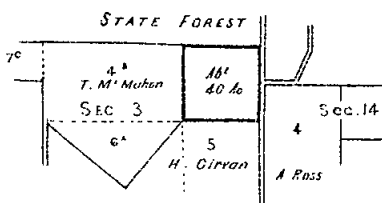
F. 70343, P. 136. Diagram N° 88 SCALE— 40 Chains to 1 Inch
