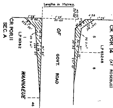
G.P. 13730 A Compiled from S.P. 13730
