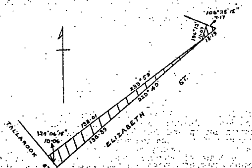
Part C.A. 14, Sec. C, Township & Parish of Seymour. Measurements in metres.
